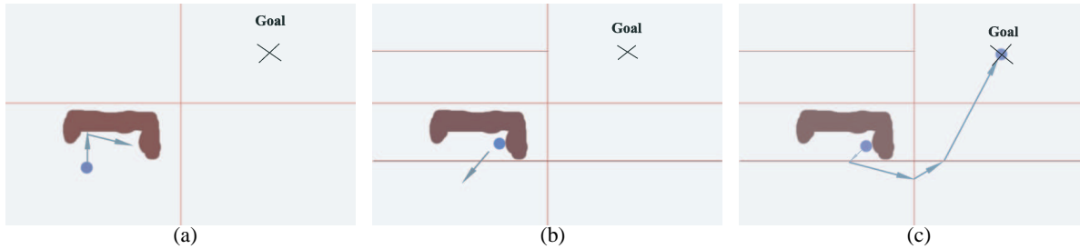
Fig. 1. Example behavior of the parti-game method
