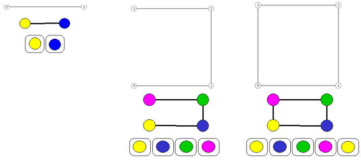
Figure 4: An example of topologies as label sequences (bottom), with each label shaded (colored) differently. Each label sequence corresponds to a set partition.
