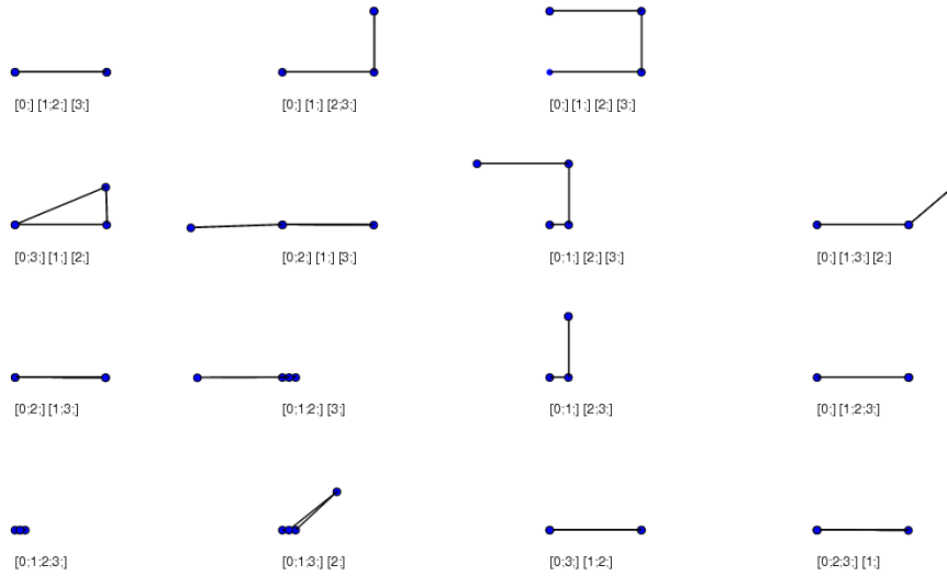
Figure 3: There are 15 possible topologies for the case of four measurements. The set partitions corresponding to the topologies are given below each topology.
