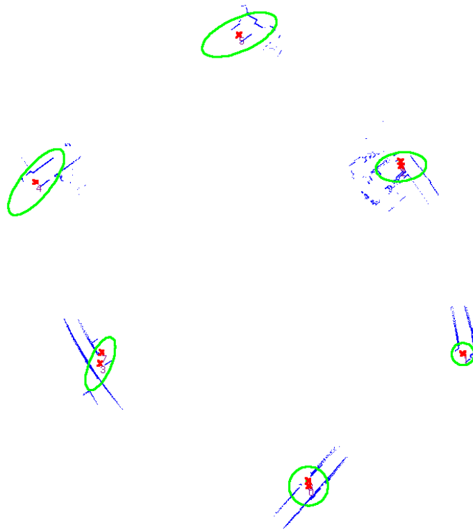
Figure 13: Maximum a posteriori sample from the RBPF for the CRB experiment. Mean landmark locations are denoted as crosses while the ellipses denote marginal covariances.
