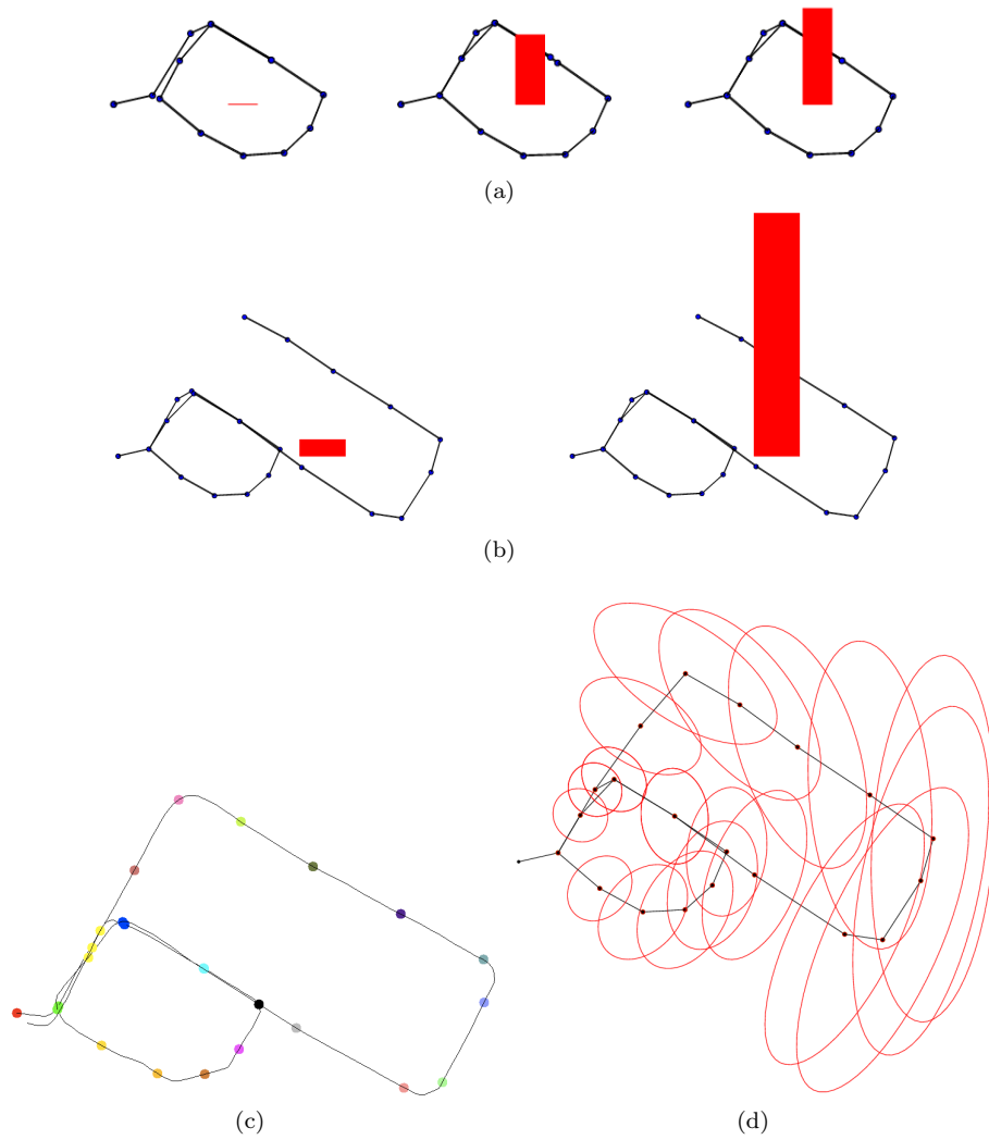
Figure 14: PTM for the TSRB dataset with 35 landmarks placed equally in time (a) PTM after 13 landmarks (b) After 29 landmarks - the difference between the topologies is in the small triangular piece at the top of the smaller loop (c) The final PTM after 35 landmarks contains only one topology, which is also the groundtruth. Landmarks are shown as small shaded (colored) circles with nodes corresponding to the same physical landmark shaded (colored) similarly (d) 5\sigma covariance ellipses for the landmark locations of the ground-truth topology.
