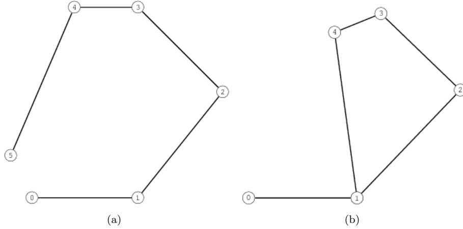
Figure 2: Two topologies with 6 observations, each corresponding to set partitions (a) with six landmarks ( \{0\}, \{1\}, \{2\}, \{3\}, \{4\}, \{5\} ) and (b) with five landmarks ( \{0\}, \{1, 5\}, \{2\}, \{3\}, \{4\} ), illustrate the equivalence between topologies and set partitions.
