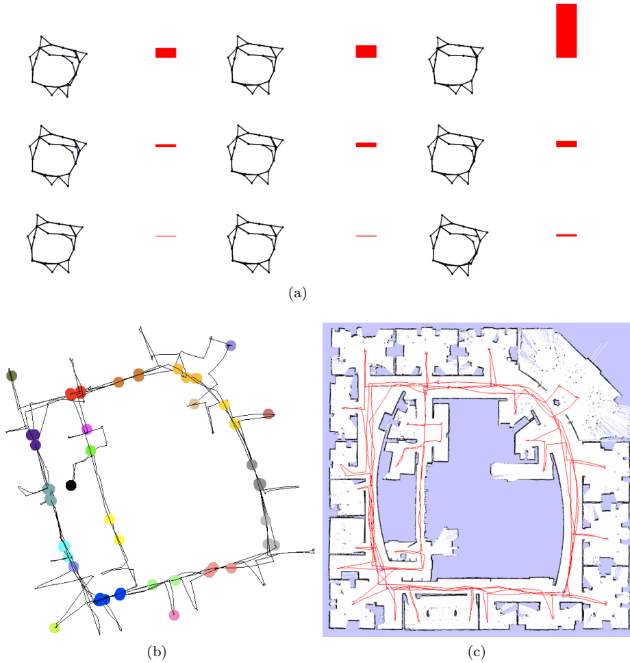
Figure 1: (a) PTM (Bayesian posterior over loop closings) for the Intel dataset obtained using the OPTM algorithm. 63 landmarks were placed in the environment at a distance of 5 meters from each other. The bars give the posterior probability of each topology (b) Smoothed trajectory for the most likely topology, which is also the groundtruth topology and gets 72% of the probability mass. Landmarks are shown as shaded (colored) circles with nodes corresponding to the same physical landmark shaded (colored) similarly (c) Metric map of the Intel lab given for reference.
