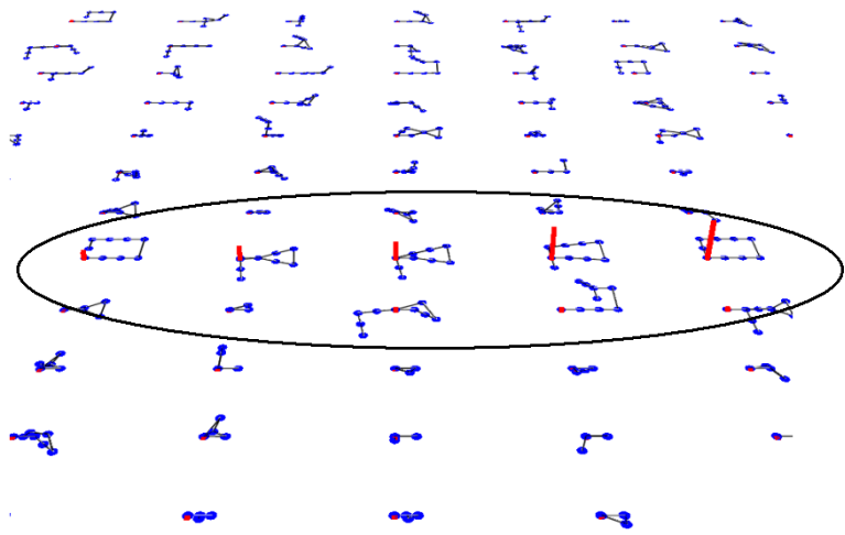
Figure 5: Even though the space of topologies is combinatorial, topologies with non-negligible probabilities are relatively few and localized. A portion of the space of topologies obtained with ten observed landmarks is shown. The groundtruth is the topology with the highest probability
