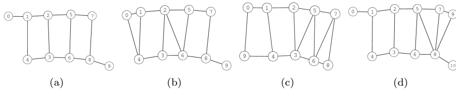
Figure 10: Topologies with highest posterior probability mass for the second experiment. (a) the ground truth topology receives 59% of the probability mass while (b), (c), and (d) receive 9.1%, 8.2%, and 6% of the probability mass respectively.
