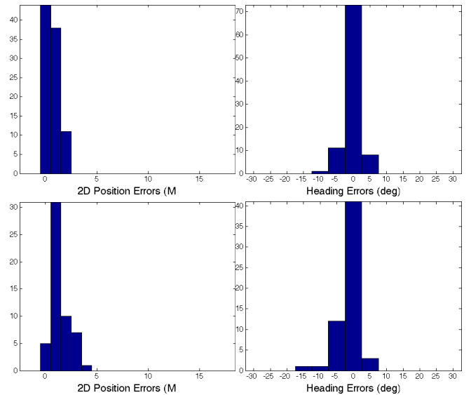
Fig. 8. Histograms of 2D position error and heading error for localizing using road marks under the same test conditions as the template images (top) and different test conditions (bottom). Accuracy is much higher than for map-based localization in both cases and accuracy is maintained across the two cases. The number of detections and pose estimation also does not drop as drastically as with map-based localization. Y-axis of the histograms represents pose estimation count.
